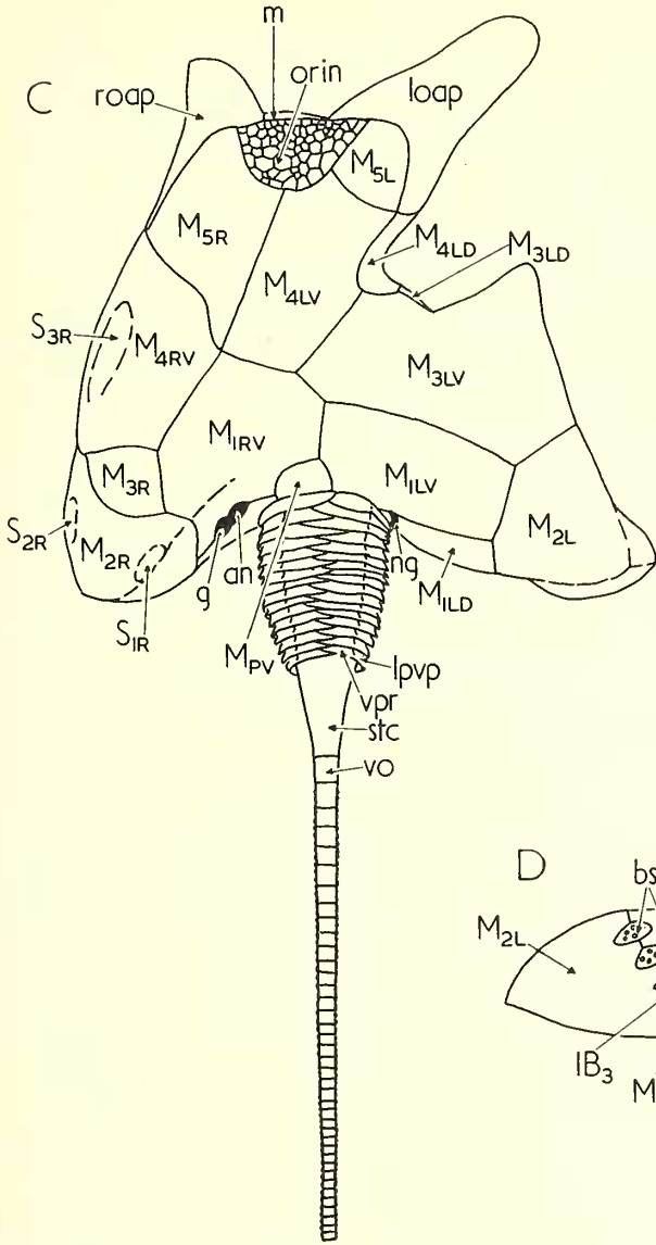
TEXT-FIG. 2. Ceratocystis perneri Jaekel. Reconstruction of external features. A, dorsal; B, right lateral; C, ventral; D, posterior aspects. For plate and spike notation, see text. ag = accessory gaps; an = anus; as = anterior stem; bs = branchial slit; dg = dorsal groove (median eye); g = gonopore; h = hydro-pore; loap = left oral appendage; lpvp = lateral portion of a ventral anterior stem plate; m = mouth; ng = narrow groove (lateral line); or in = oral integument; ps = posterior stem; roap = right oral appendage; stc = stylocone; vo = ventral ossicle; vpr = ventral process of a ventral anterior stem plate.
